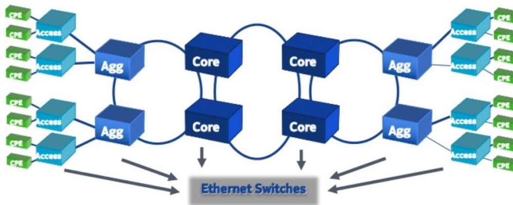
Figure 3.24 Topology of active fibre networks
