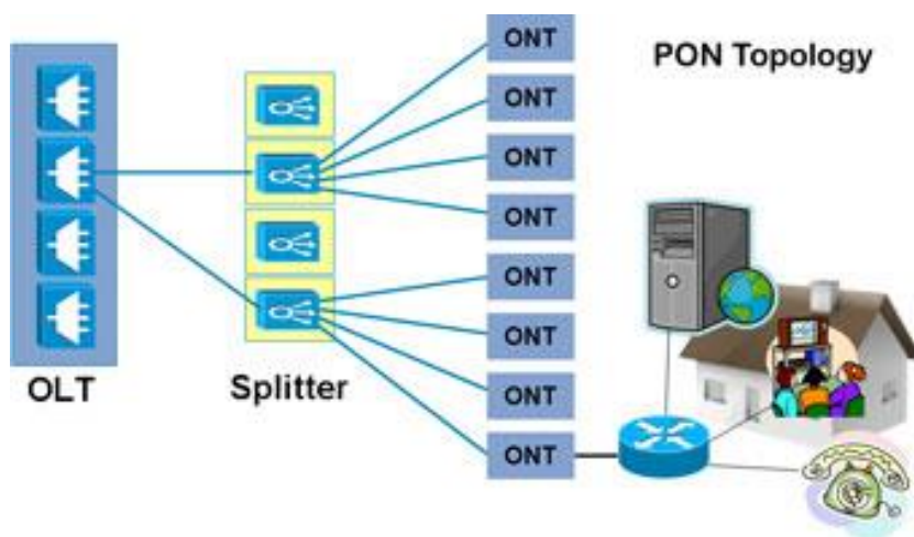
Figure 3.23 Topology of PON fibre networks
